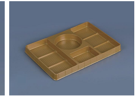
TMLH-3621 Weight:36g Material:PET Size:275*190*21mm
