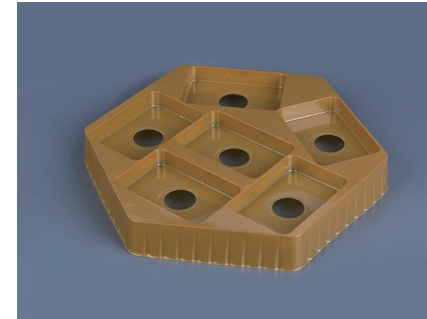
TMLH-4737.6 Weight:41g Material:PET Size:304.4*267.5*37.6mm
