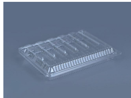
TMLD-4540 Weight:45g Material:PET Size:230*169*40mm
