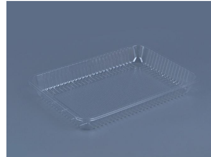
TMHB-11.525 Weight:11.5g Material:PET Size:205*140*25mm
