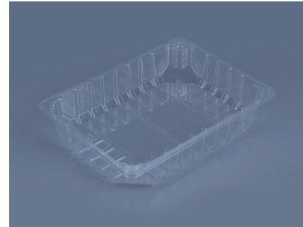
TMSX-3740 Weight:37g Material:PET Size:276.98*203.98*40±1mm
